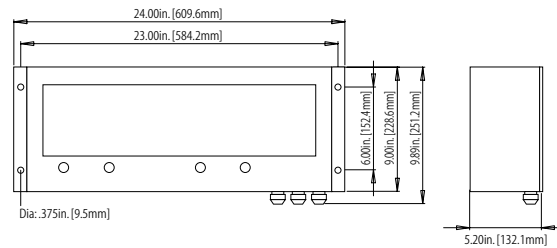
XR 4500TL/XR6500
